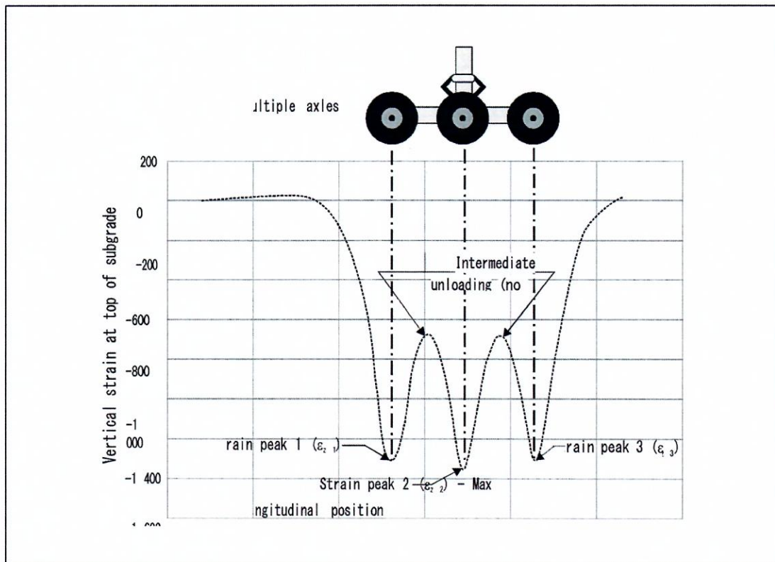
Figure A3-1.Example of multiple-axle gear strain response
