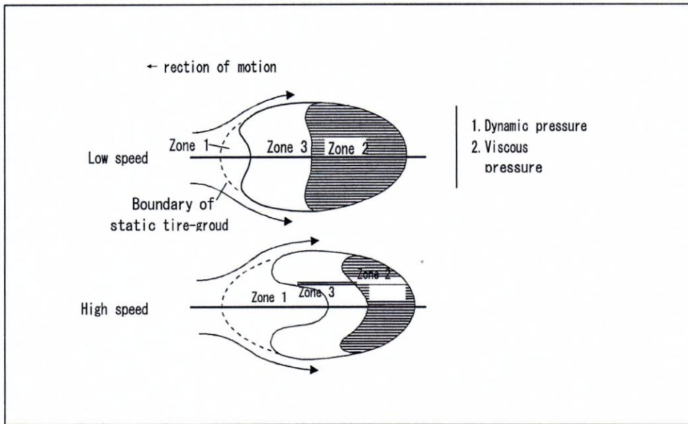
Figure A6-2.Areas of tire/surface interface
