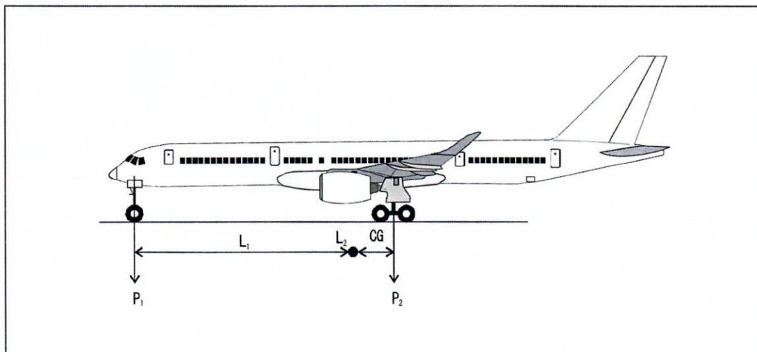
Figure A1-1. Aircraft weight distribution on ground
