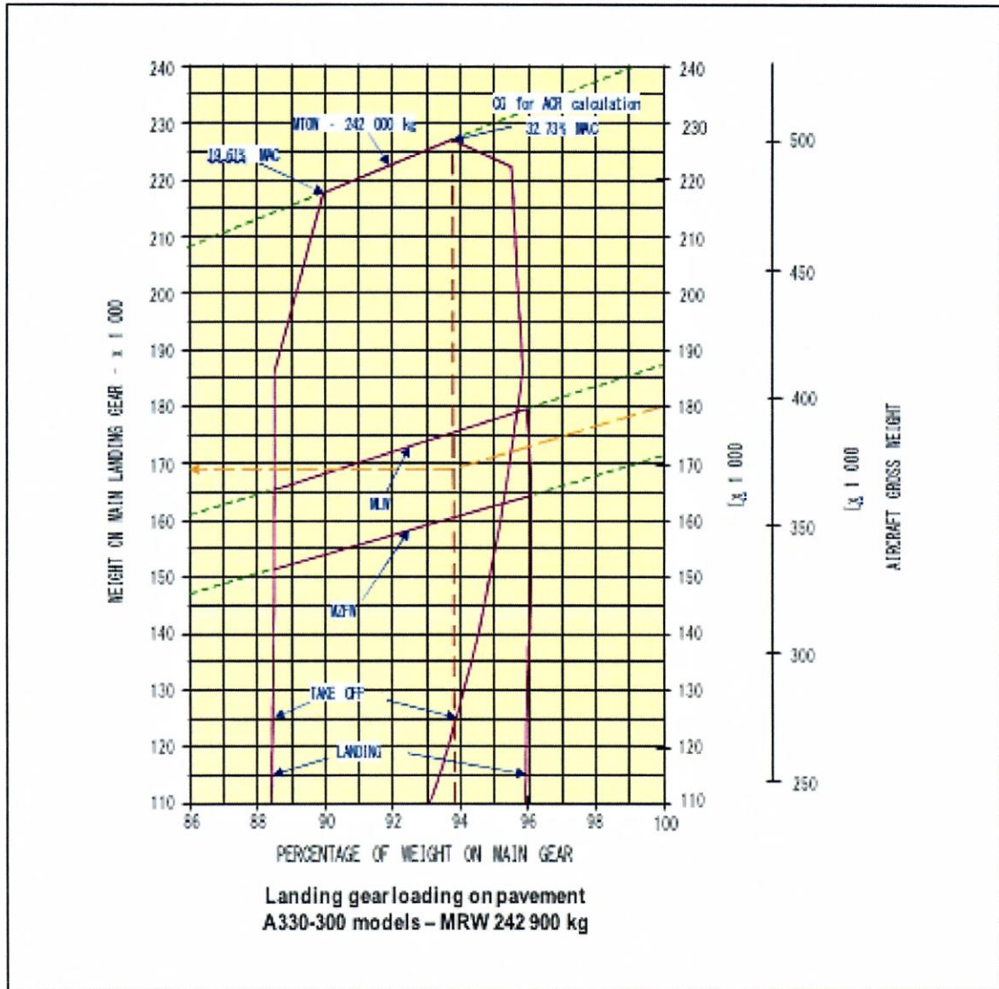
Figure 1-3. Landing gear loading on pavement – Airbus A330-300
