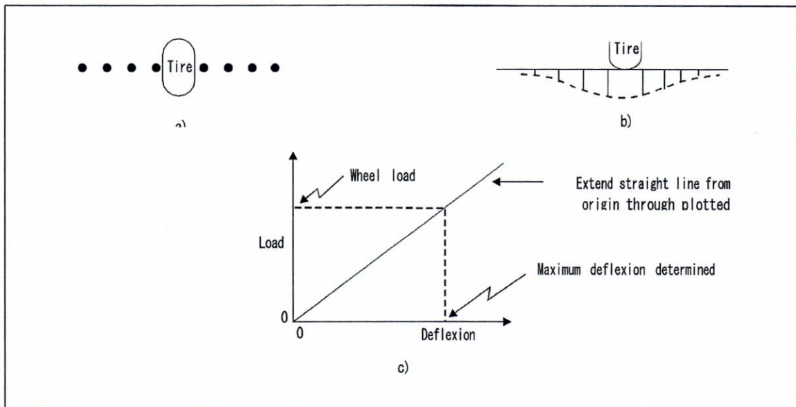
Figure 3-4.Relation between load and deflection
