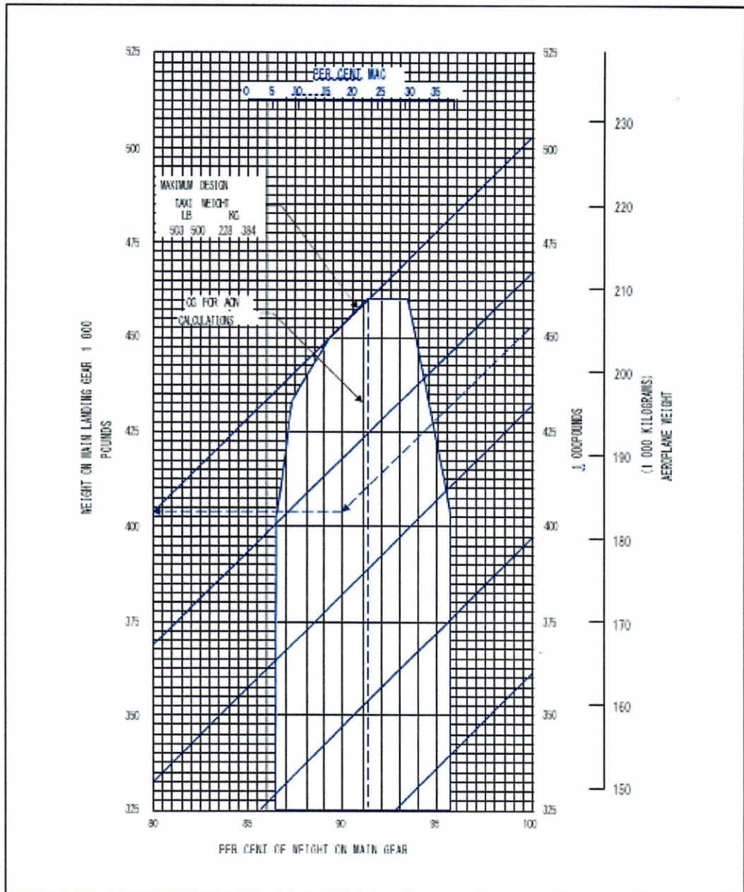
Figure 1-4. Landing gear loading on pavement – Boeing 787-8
