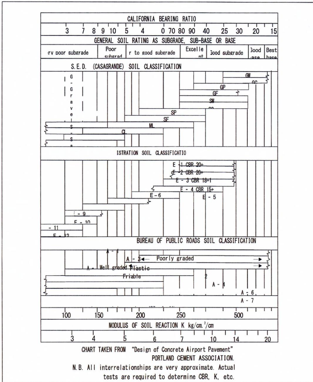
Figure 3-2. Interrelationships of soil classification, California Bearing Ratio (CBR) and k value
