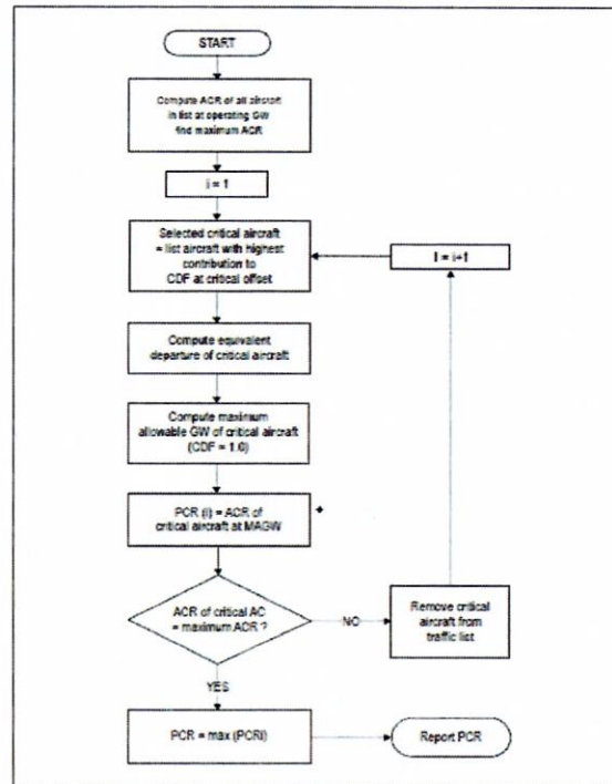
Figure 1-9. Flowchart of recommended PCR computation procedure
