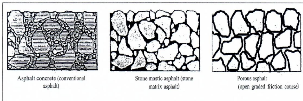
Figure A6-12. Asphalt concrete versus SMA versus porous asphalt
