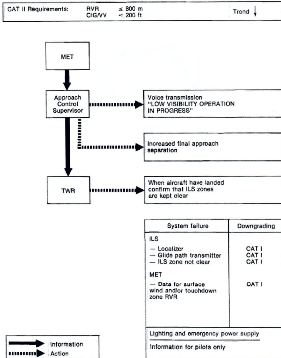
Figure B-4. All weather operations - Frankfurt-Main Airport (Category II operations)
