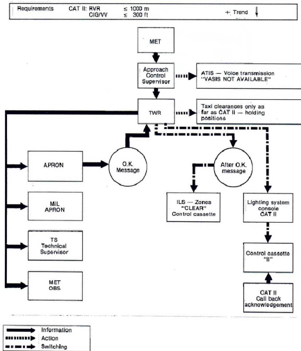
Figure B-3. All weather operations - Frankfurt-Main Airport (Category II/III operations)
