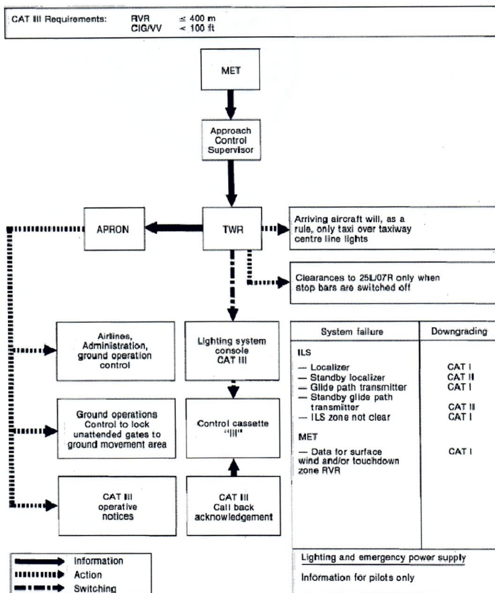
Figure B-5. All weather operations - Frankfurt-Main Airport (Category 111 operations)
